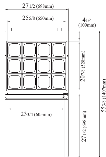
TOP VIEW
